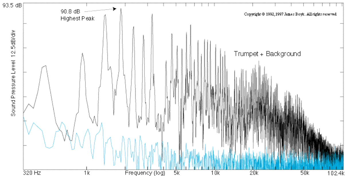
Figure 1(a) (Amplitude vs frequency). Trumpet with Harmon mute , 95.5 dB at Aco 7016 microphone 4 feet away. Microphone aimed at bell, which was angled down about 20 degrees. Upper Trace: Trumpet + Background, corrected to 70 kHz (see text). Lower trace: Background alone.
