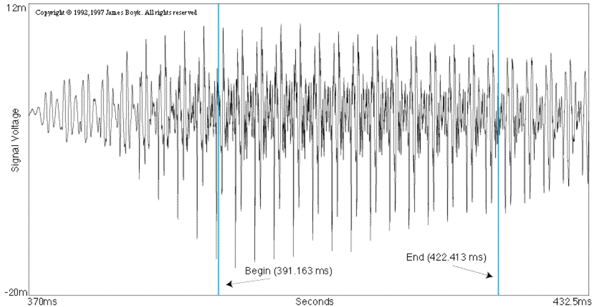
Figure 1(c) (Amplitude vs time). Trumpet with harmon mute . The time sample analyzed to make Figure 1(a). The trace shows, between the "Begin" and "End" marks, the 31.25-millisecond record from which the spectrum was created by Fourier analysis.
