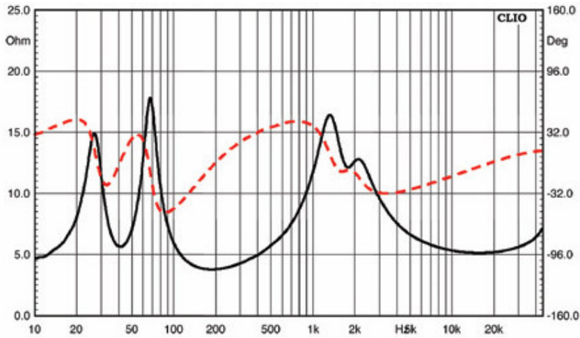
Opera Callas Impedance and Phase of Impedance (red)
